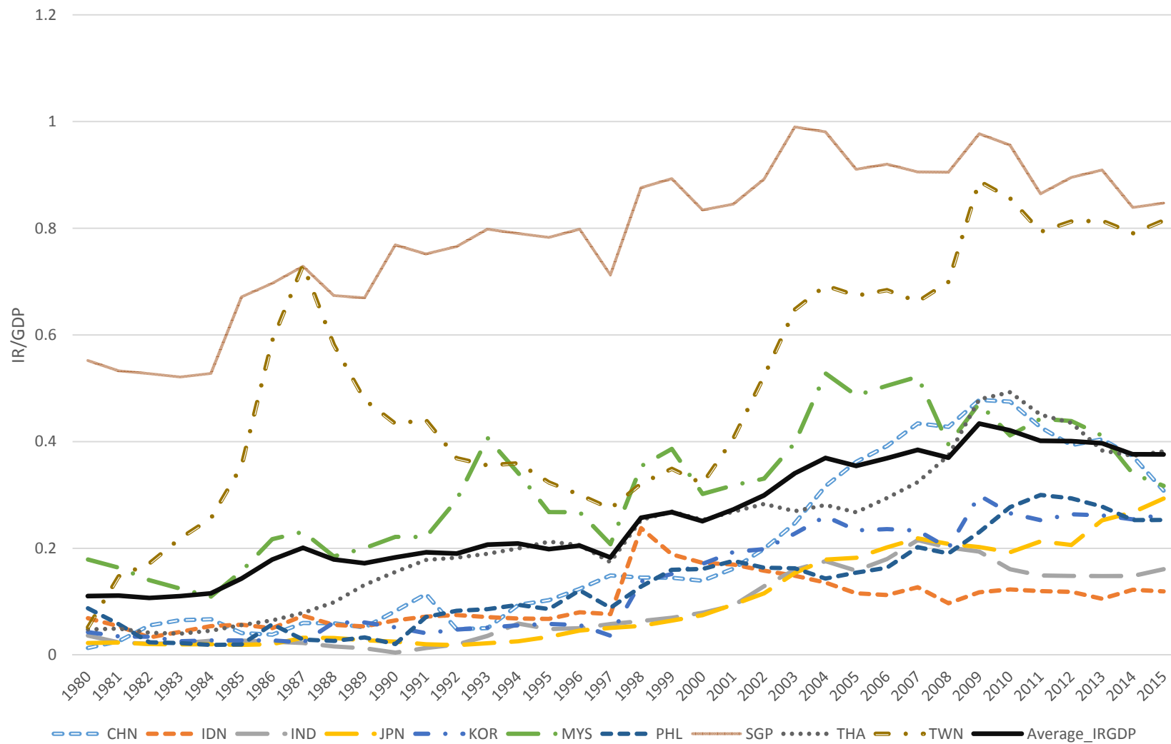
Figure 1: Ratios of international reserves to GDP: 10 Asian Economies
