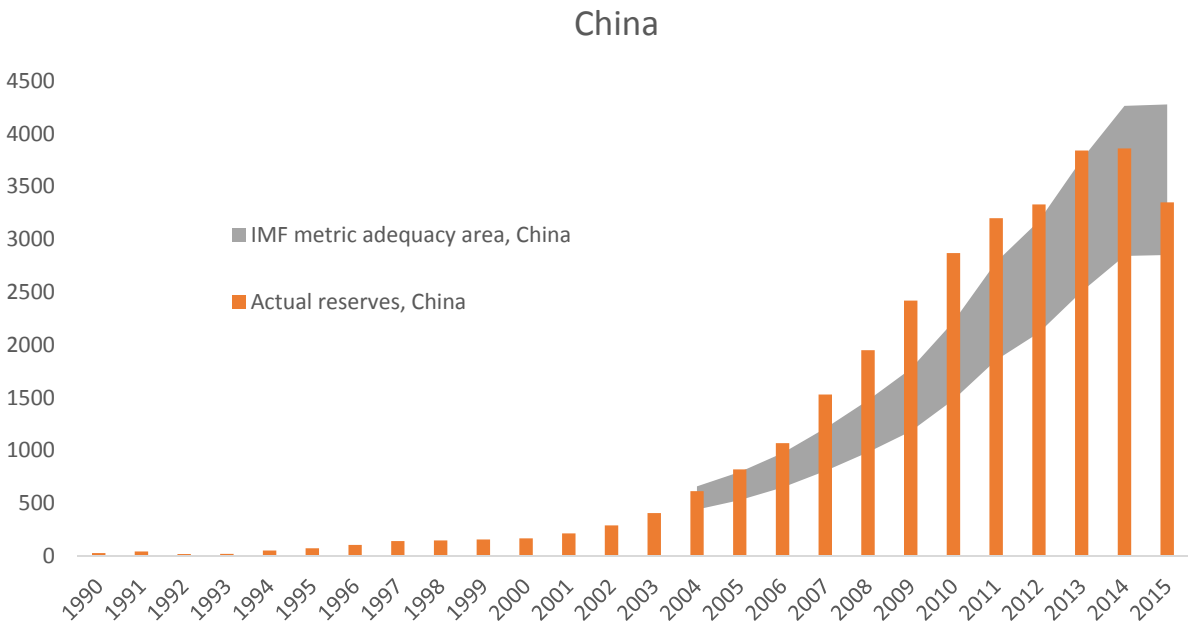
Figure 4: The IMF ARA metric prediction and the Adequacy Range, and actual holdings of International Reserves (Billions USD)
