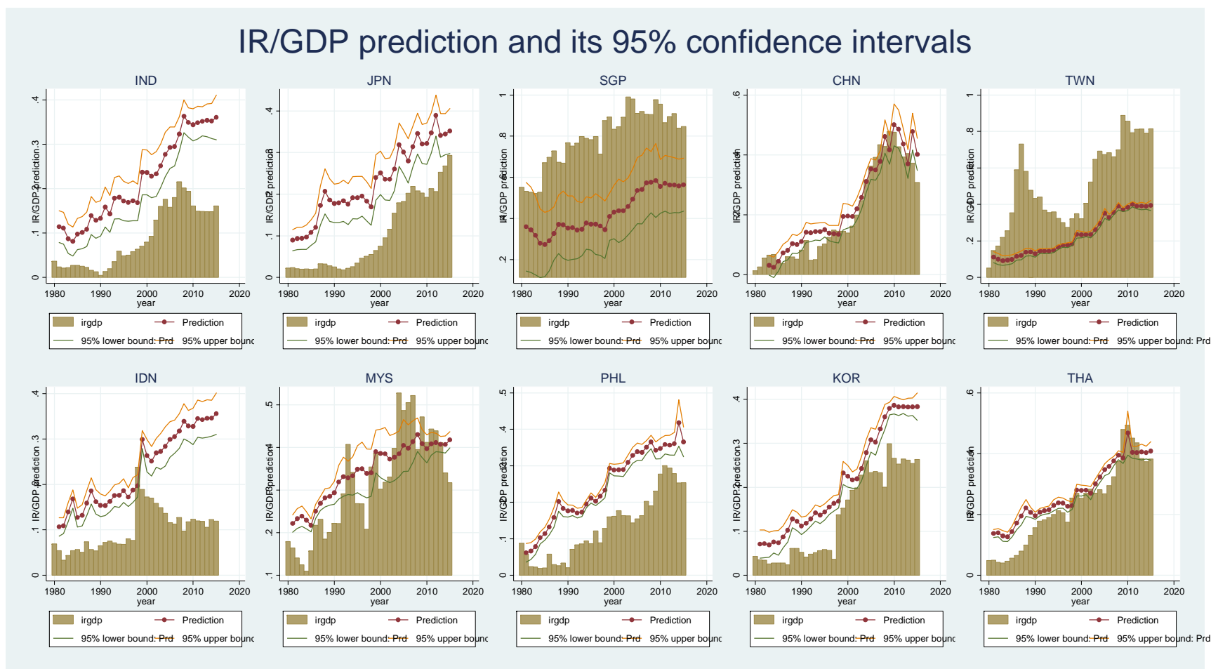
Figure 3: Comparison of IR/GDP and its prediction with 95% confidence intervals
